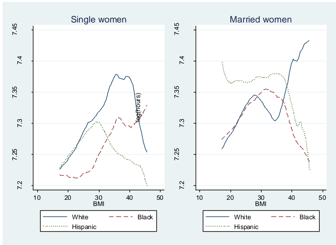
Figure 2: Semi-parametric regressions without endogeneity: association between BMI and hours worked for single and married women
