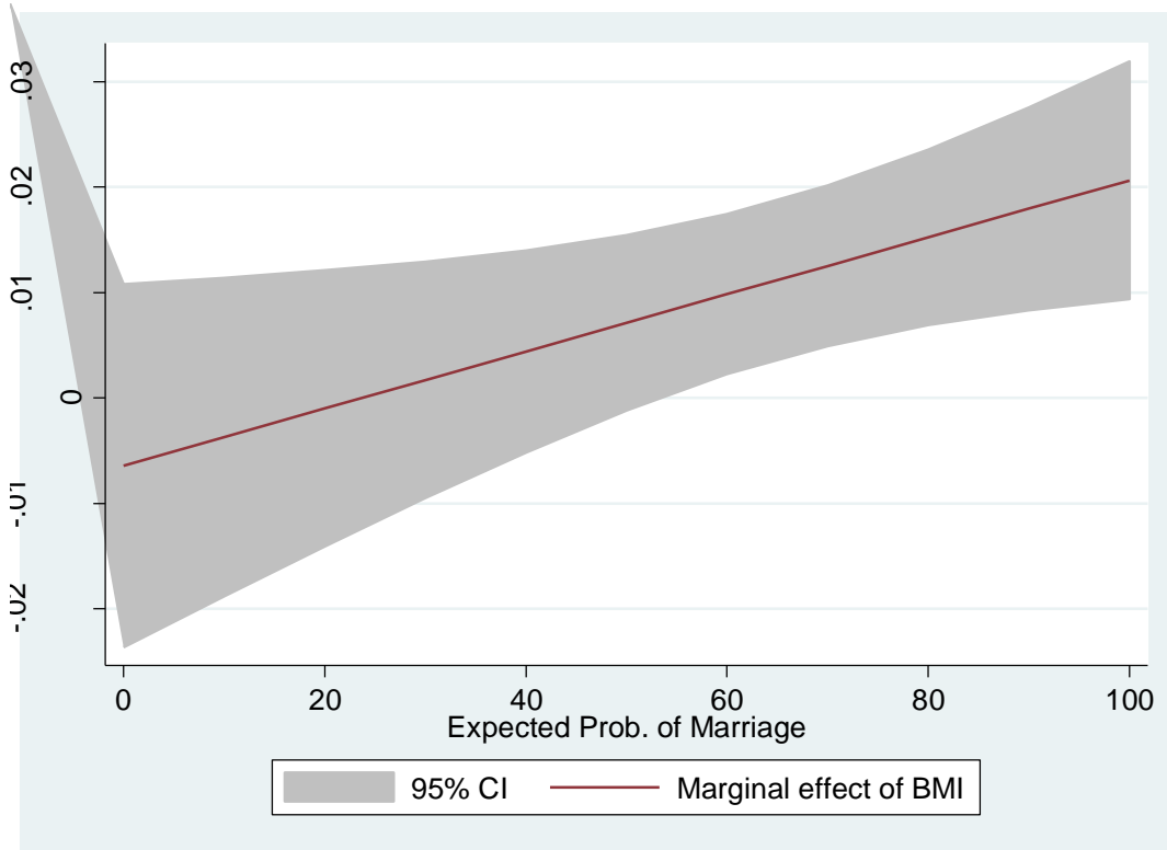
Figure 1: Effect of BMI on hours worked by single white women: by expected probability of marriage
