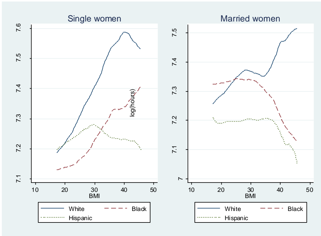
Figure 3: Semi-parametric IV regressions: effect of BMI and hours worked for single and married women
