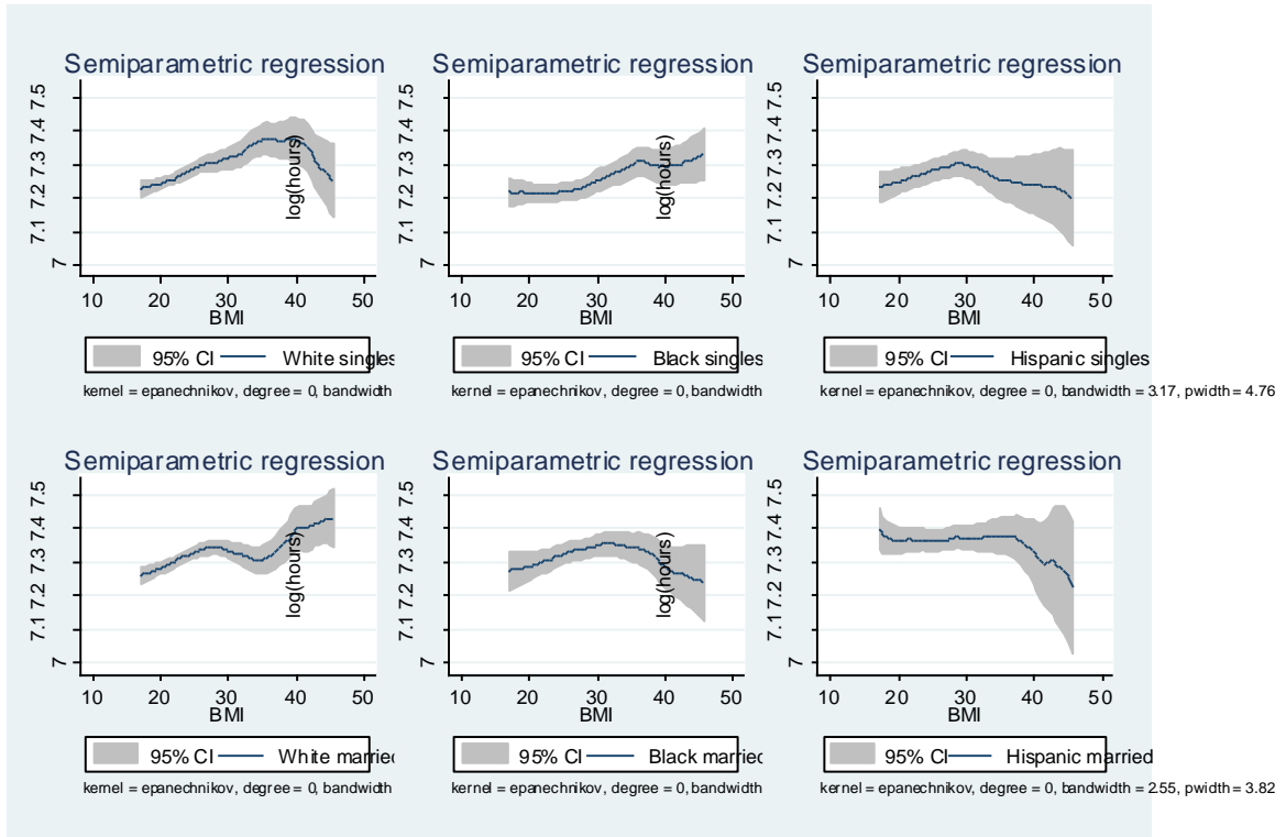
Figure A1: semi-parametric regression results with 95% CI
